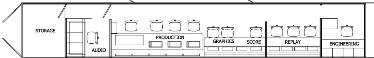
VMU (B-Unit) 53' Long, 13'3" High, 8'6" Wide
