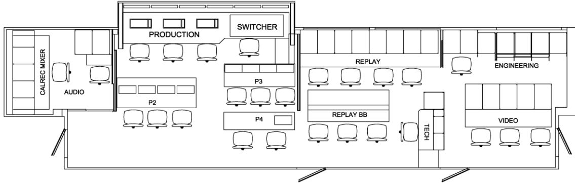
VMU (B-Unit) 53' Long, 13'3" High, 8'6" Wide
